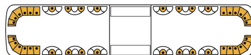
53" (1346 mm) Lightbar, amber colour, part number. 2061003PL
