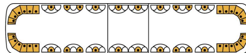
53" (1346 mm) Lightbar, amber colour, part number. 2061005PL
